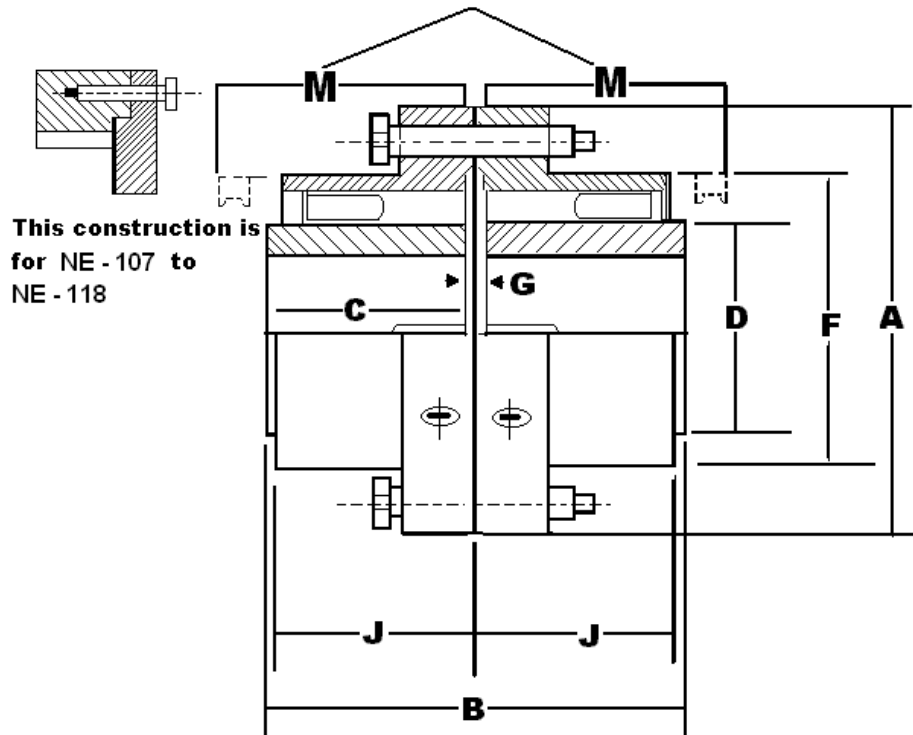
MINIMUM CLEARANCE REQUIRED FOR ALIGNING
